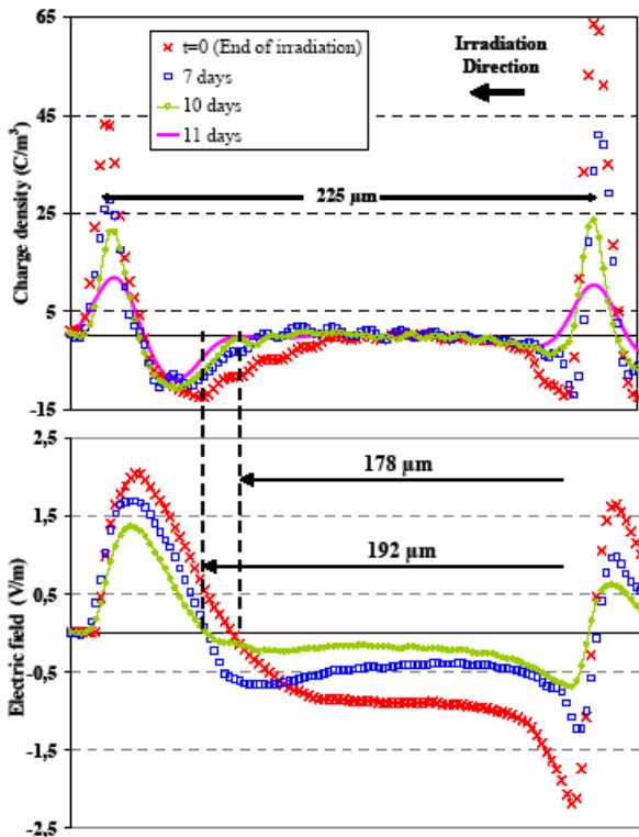
Fig. 1. Kapton sample 225 \mu\text{m} -thick charge density recorded by PEA and electric field calculated during the relaxation after 30 mn irradiation under 150 keV with a flux of 125 pA/cm 2 .
