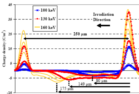
Fig. 2. PEA measurements recorded on a PMMA sample 250 \mu\text{m} -thick during three periods of 40 mn irradiation a) 100 (crosses), b) 130 (open circle) and c) 160 keV (single line) with a flux of 50 pA/cm 2 .
