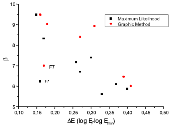
Fig. 1. Relation between \beta and (\log E_\gamma - \log E_{\beta_{min}}) for the formulations.
