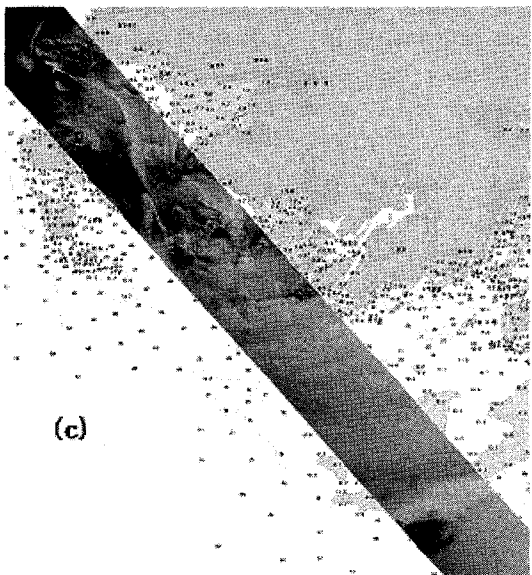
Fig. 2 X-SAR image acquired (a) at 12:44:33 on April 15 (b) at 12:24:09 on April 16 (c) at 12:36:02 on October 7, 1994.
