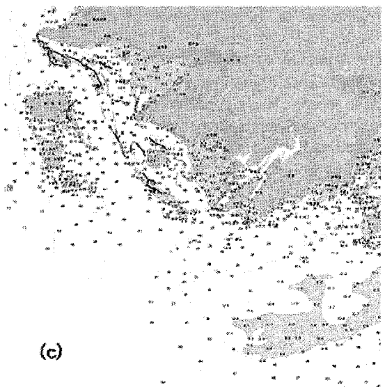
Fig. 3 Overlapping the bathymetry with the signatures on the SAR image (a), (b), and (c) in Fig. 2
