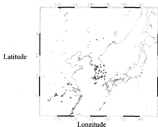
Fig. 1. Location of observation stations over Korean peninsula
