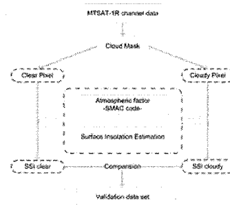
Fig. 2. Algorithm for the Surface Solar Insolation
