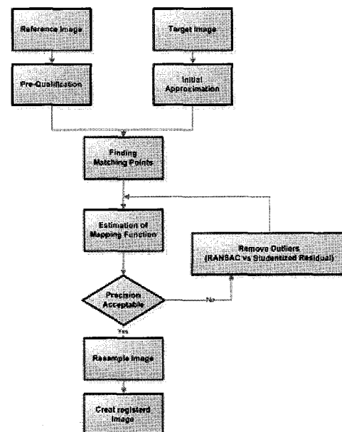
Figure 1. The Flow Chart of Pre-Qualified Area Based Matching
