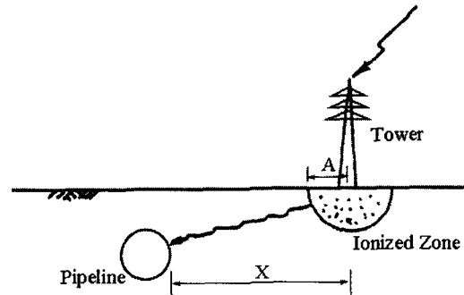
Fig. 1. Arcing from a tower to a pipeline through the soil
