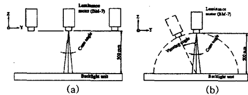
Fig. 4 A measurement method of (a) spatial luminance and (b) angular luminance
