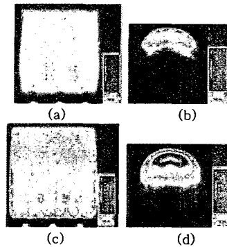
Fig. 5 A simulation result of (a), (c) spatial luminance and (b),(d) angular luminance in (a), (b) positive and (c) (d) negative micro-lens patterned LGP (h = 15 um)
