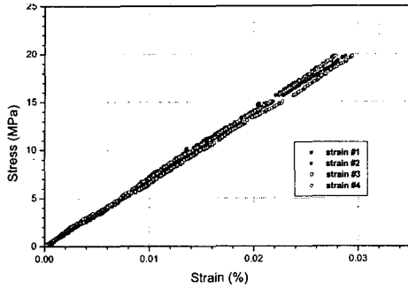
Fig. 7 Test results using Chain and Rubber Pad
