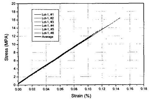
Fig. 10 Test Results of Six Specimens
