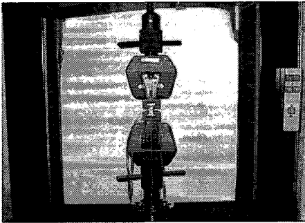
Fig. 2 Test Fixture using Grip
