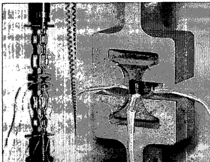
Fig. 8 Test Fixture of Composite Specimen
