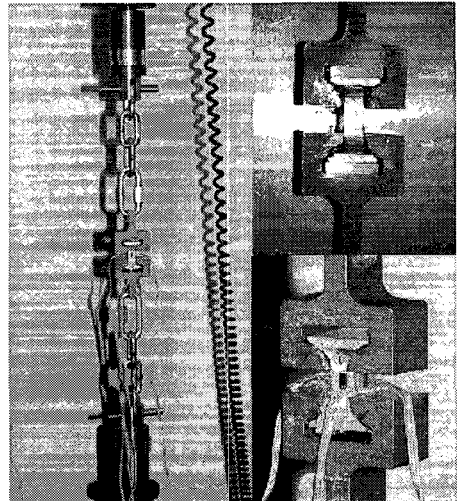
Fig. 6 Test Fixture using Chain and Rubber Pad
