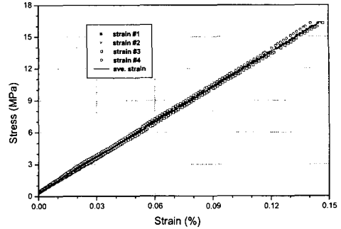
Fig. 9 Test Results of Composite Specimen
