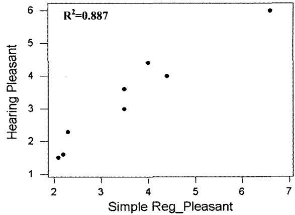
(a) Simple regression output
