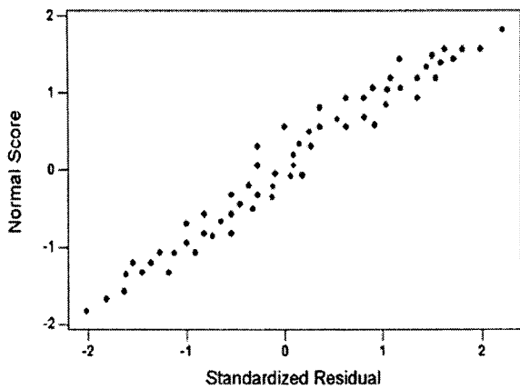
(a) Testing for the normality
