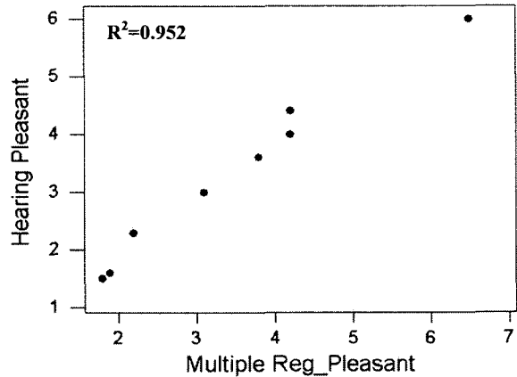
(b) Multiple regression output
