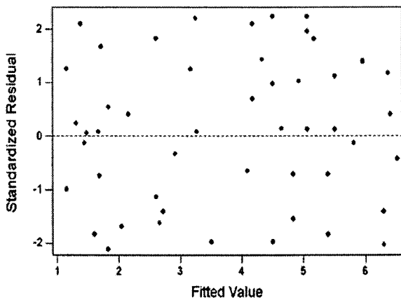
(b) Testing for homoscedasticity
