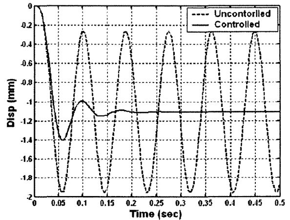
(a) Impulse response
