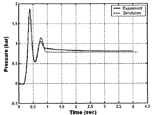
(b) Comparison between experimental and analysis results
