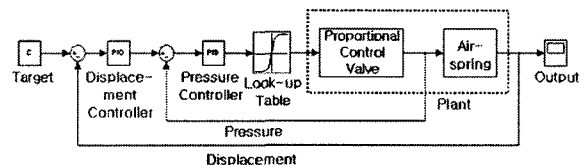
Fig. 4 Block diagram of air-spring control system
