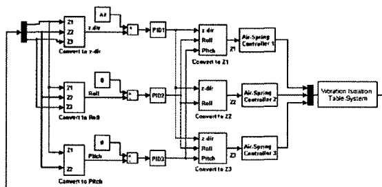
Fig. 6 Block diagram of mode-based control system
