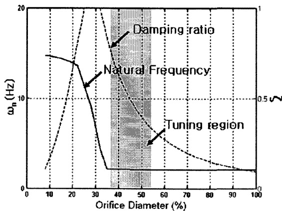
Fig. 3 Analysis of natural frequency and damping ratio
