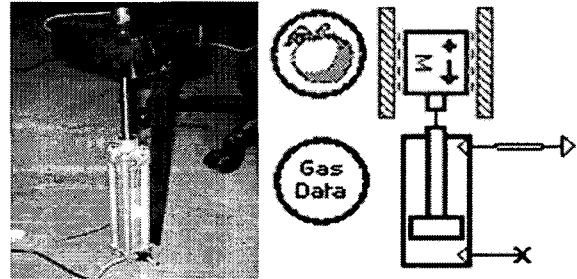
(a) Pneumatic cylinder and modeling with AMESim
