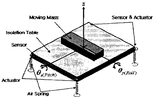
Fig. 5 Active vibration isolation system model
