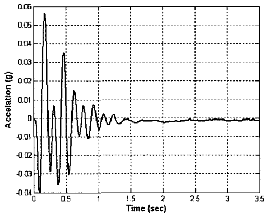
(a) Impulse Response (z-dir)
