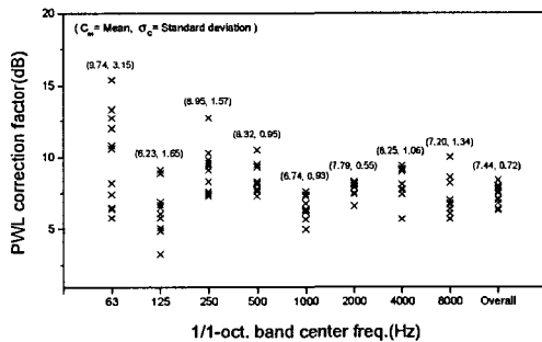
Fig. 7 Distribution of PWL correction factor for a large bus
