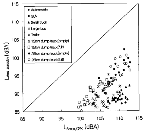
Fig. 6 Measured L_{Aeq,CPX} and L_{Amax,passby}
