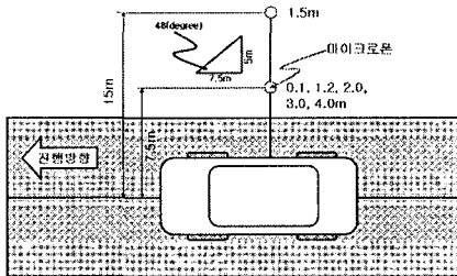
Fig. 2 Microphone positions at the pass-by measurement
