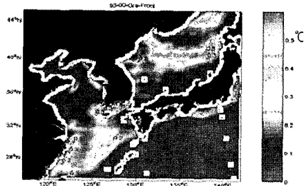
Fig. 5. Distributions of SST gradient value (°C) and Thermal Fronts (red dotted line) [9].
