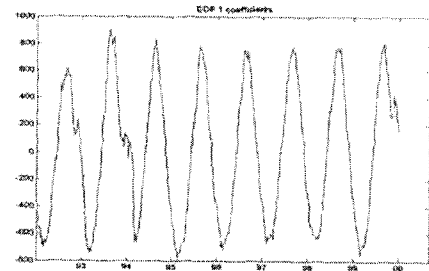
Fig. 3. The 1st mode of SST for temporal variations.
