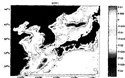
Fig. 7. The 1st mode of SST gradient for spatial distributions.
