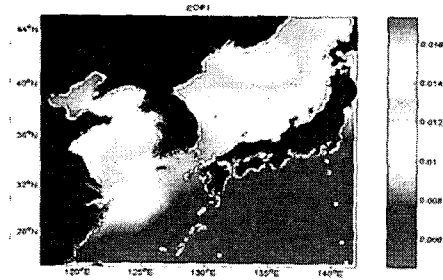
Fig. 2. The 1st mode of SST for spatial distributions.
