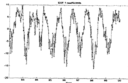
Fig. 8. The 1st mode of SST gradient for temporal variations.
