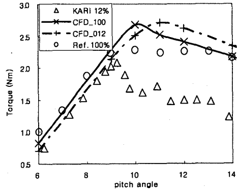
Fig. 9 Wind turbine scale effect
