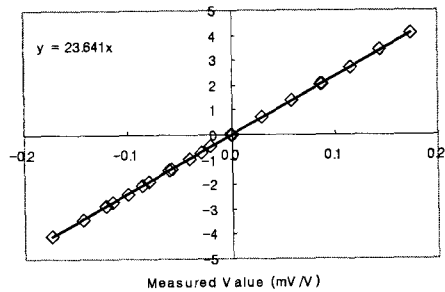
Fig. 5 Torque sensor calibration results
