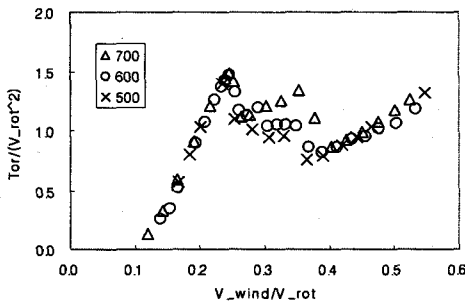
Fig. 8 Wind turbine RPM effect
