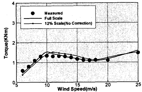
Fig. 1 Wind Turbine scale effect by CFD
