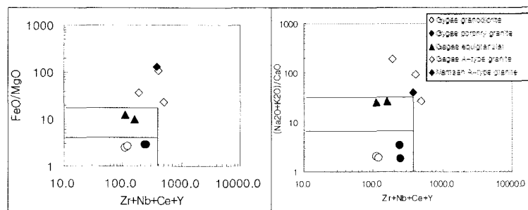
Fig. 2. FeO/MgO vs Zr+Nb+Ce+Y and (Na_2O+K_2O)/CaO vs Zr+Nb+Ce+Y diagrams of the Kigae and Namsan granitic rocks(Whalen et al., 1987) Symbole : FG=fractionated felsic granites, OGT=unfractionated orogenic M-, I-, S-type granites, A=felsic A-type granite average in Australia, I=felsic I-type granite average in Australia, S=felsic S-type granite average in Australia.
