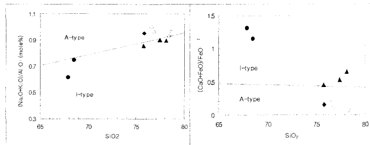
Fig. 3. (Na_2O+K_2O)/Al_2O_3 vs. SiO_2 and (CaO+MgO)/FeO vs SiO_2 diagram for the Kigae and Namsan granite. Symbole are the same as those Fig. 2.
