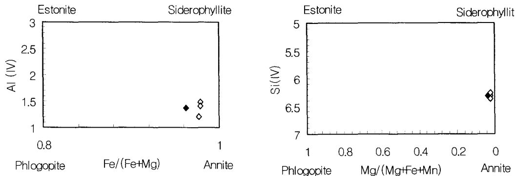
Fig. 5. Chemical compositions of biotite plottes plotted in Si(IV) vs, Mg/(Mg+Fe+Mn) and Al(IV) vs, Fe/(Fe+Mg). Symbols are same as Fig. 2.
