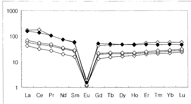
Fig. 4. Chondrite anormalized REE abundances pattern diagram(Sun, 1982). Symbole are the same as those Fig. 2.
