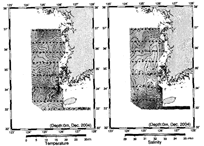
Fig. 4. In-situ temperature(left) and salinity(right) distributions at the depth 0m in Dec. 2004.
