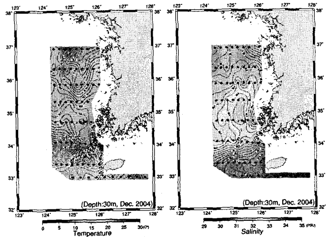
Fig. 5. Same as for Figure 4 but for the depth 30m in Dec. 2004.
