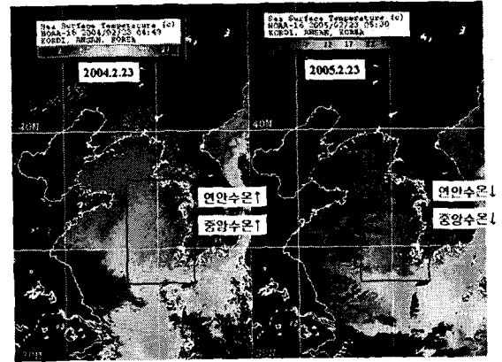
Fig. 3. SST images of NOAA for the season winter of 2003 and 2004.
