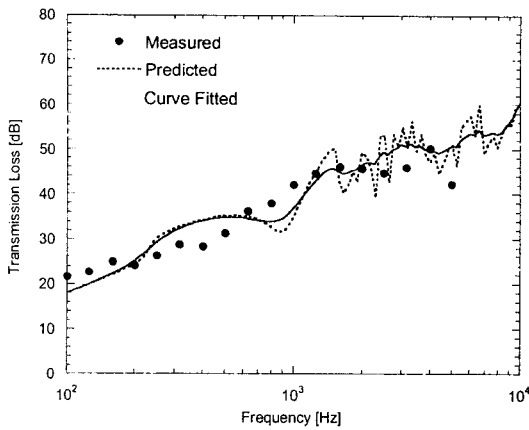
Fig. 7 Predicted and measured transmission loss of dash panel
