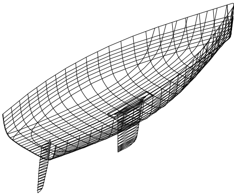
Fig.3 Designed hull form
