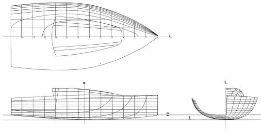
Fig.2 Lines of parent ship
