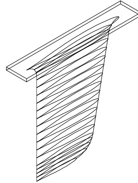
Fig.6 Designed keel
