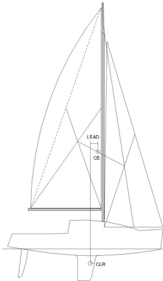
Fig.7 Locations of CE, CLR and lead
