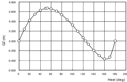
Fig.5 Righting moment arm (GZ)
