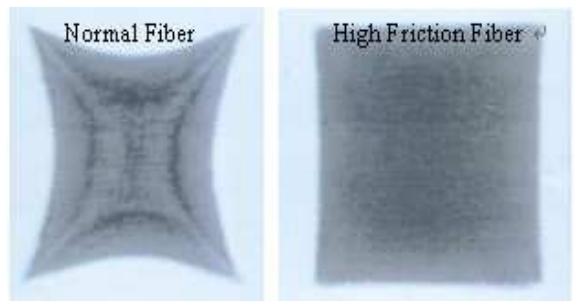
Fig. 6. NDI C-scan of honeycomb sandwich core
