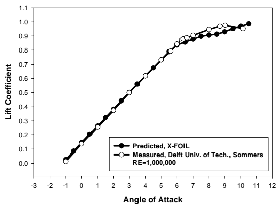
Fig. 1 Lift coefficient comparison (S809)
