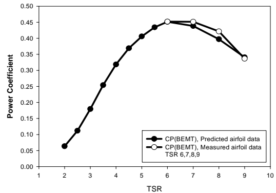
Fig. 2 Comparison of the power coefficient on the FIL-20
