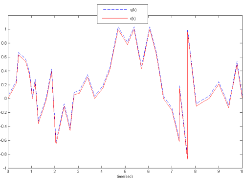
Fig. 6. The simulation result of the DTFEL system with PD controller with system disturbance.
