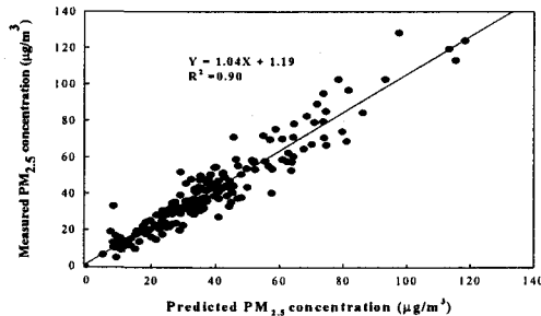
Fig. 2. Measured versus predicted PM 2.5 mass concentration.
