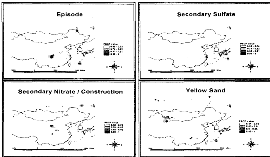
Fig. 3. Possible Source Locations for resolved PMF model using PSCF.
