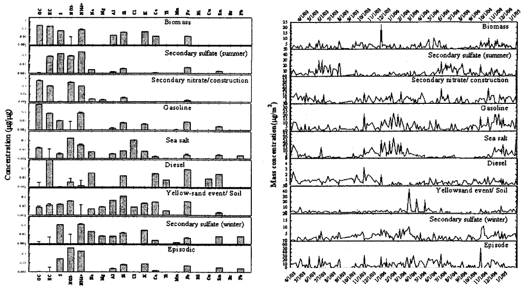
Fig. 1. Source profiles and contributions resolved from PM 2.5 samples
