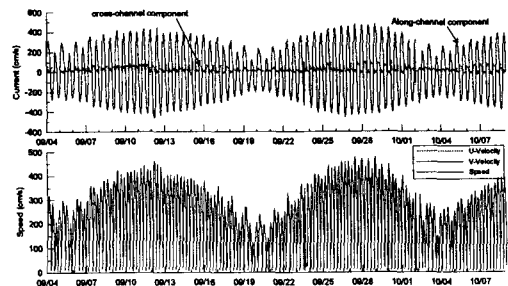
Fig. 2 Along and cross-channel component of depth-averaged current (upper) and temporal variation of current speed (lower).
