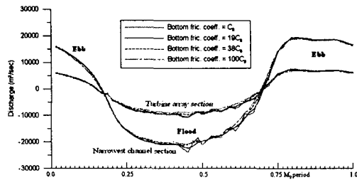
Fig. 8 Discharge change through the narrowest channel and turbine Array section due to turbine operation.
