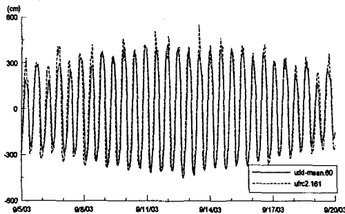
Fig. 4 Result of validation using the depth-averaged ADCP current data measured during September, 2003 (solid: measured, dotted: computed).
