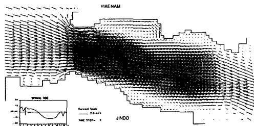
Fig. 7 Computed ebb current after reclamation.
