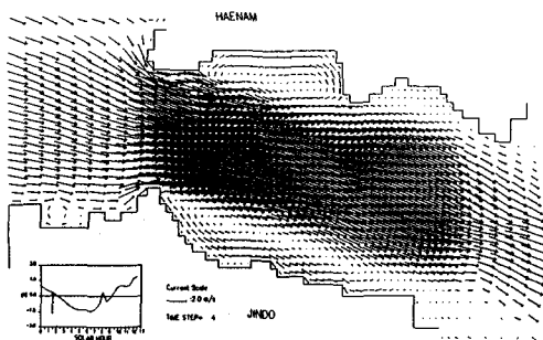
Fig. 5 Computed ebb current field around the narrowest channel in the Uldolmok.
