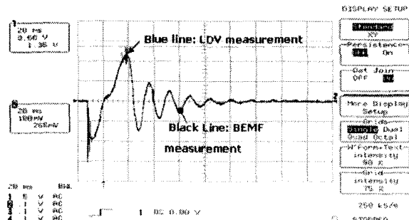
Fig. 3 Velocity detection in focusing direction : LDV vs. Back EMF
