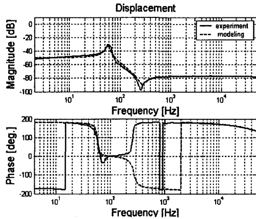
Fig. 7 FRF G_{21}(s) from focusing input to tracking output
