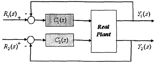
Fig. 8 Closed loop configuration for 2 by 2 system
