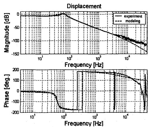
Fig. 2(b) FRF for tracking direction
