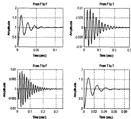
Fig. 11 Step response for decoupled system
