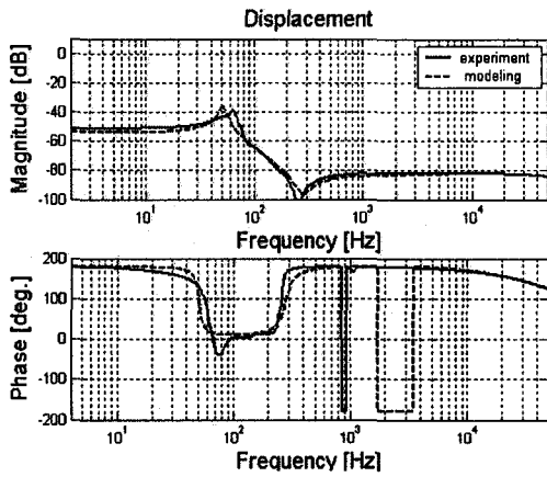
Fig. 6 FRF G_{12}(s) from focusing input to tracking output
