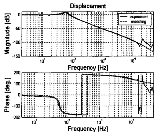
Fig. 2(a) FRF for focusing direction
