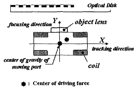
Fig. 4 Side view of moving part
