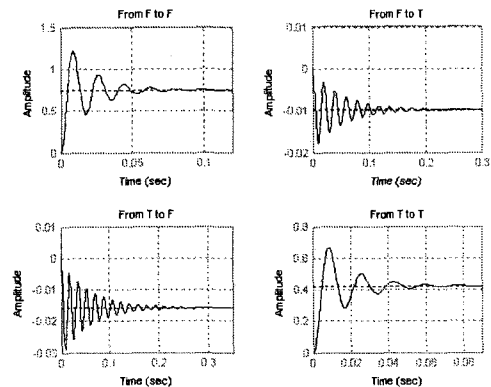
Fig. 10 Step response each transfer function for G(s)
