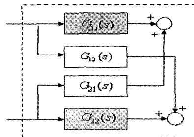
Fig. 5 Diagram for interacting MIMO system
