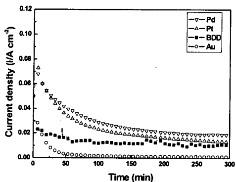
Figure 2. Current-time profile of Pd, Pt, BDD and Au electrode at applied potential of + 1.54 V (vs. H/HgO) and NaBO 2 solution of 20 wt. % for 5hours.
