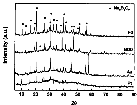
Figure 3. XRD analysis of electrochemical product from NaBO 2 aqueous solution of 20 wt. % for Pd, BDD, Au and Pt electrode at + 1.54 V(vs. Hg/HgO)
