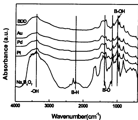
Figure 4. FT-IR data of power precipitated in a cell on BDD, Au, Pd and Pt electrode at applied potential of + 1.54 V( vs. Hg/HgO) and NaBO 2 solution of 20 wt.% for 5hours.
