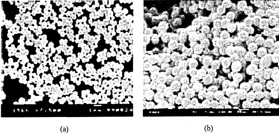
Fig. 7. Scanning electron microscopic view of food flavor nano capsules by in-situ polymerization (a) and PCM nano capsules by miniemulsion polymerization(b).
