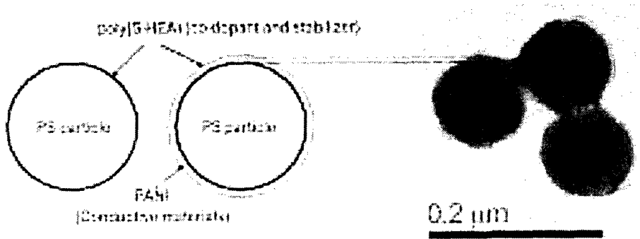
Fig. 1. Schematic drawing and TEM view of PSPEA-PANI-PSHEA-PS nano particles.
