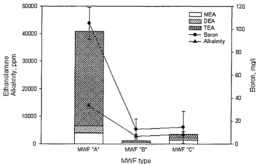
Fig. 1. Comparison of boron, alkalinity and Eas by MWF type and sump (MT01 ; MWF "A", NC01 & NC02 ; MWF "B", MT02, ML04, ML06 & DM10; MWF "C").
