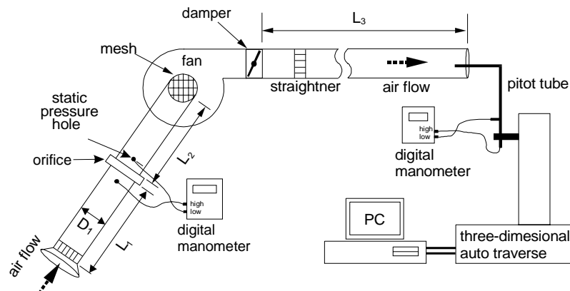
Fig. 2 Schematic diagram of experiment set-up.
