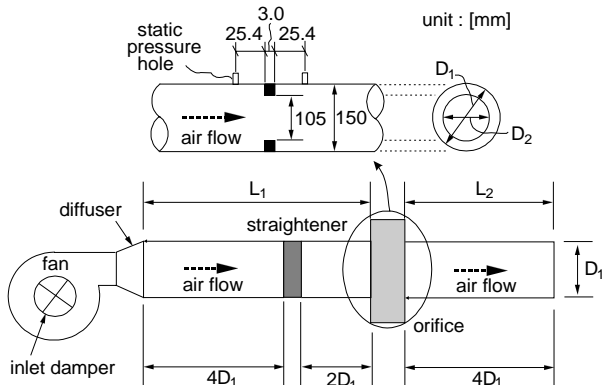
Fig. 1 Flow measuring system of duct leakage tester.
