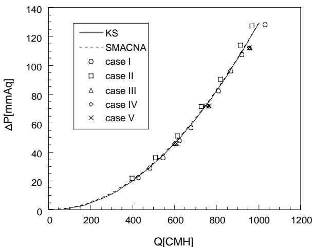
Fig. 4 Comparison of \Delta P - Q from KS standard and experiments.
