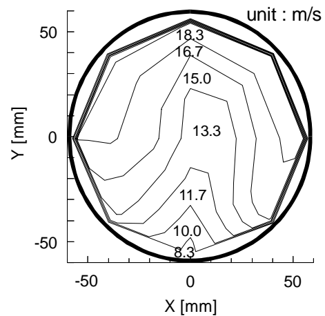
Fig. 3 Normal velocity distribution in the section of fan outlet.
