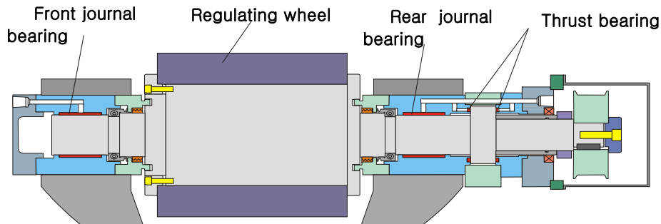
Fig. 3 Layout of regulating wheel spindle
