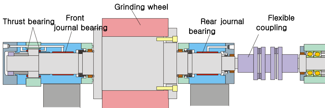
Fig. 2 Layout of grinding wheel spindle
