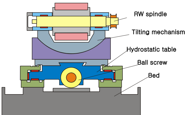
Fig. 4 Regulating wheel slide base
