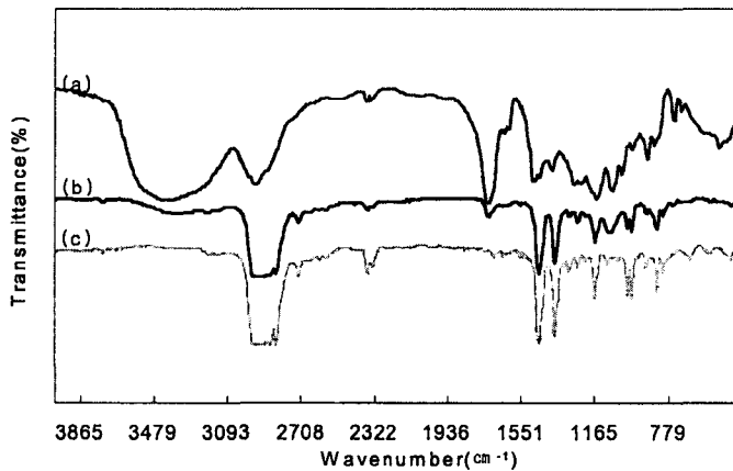
Fig. 3. FT-IR spectra (a) VBTAC + HEMA (b) Grafted PP membrane (20% grafted) (c) Original PP membrane
