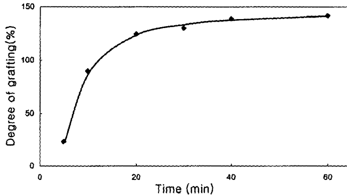
Fig. 4. Degree of grafting by UV-irradiation time
