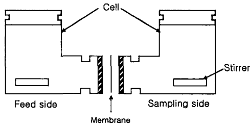
Fig. 2. Schematic diagram of permeable cell
