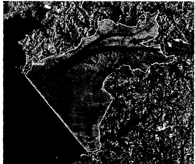
Fig. 2. DInSAR measurement of subsidence rate from zero (red) to 3cm per month (blue) obtained from Radarsat-1 InSAR pair acquired at September 27 and October 21, 2003, overlying time-averaged SAR amplitude image (16km × 15km). Maximum subsidence rate occurs at lower part of mudflat possibly due to lower supply of surface or ground water, finer mud composition, or thicker mud volume (equivalently, deeper subsurface bedrock). Note the lower subsidence rate along the river or drainage system due to constant surface water supply preventing volume contraction of mud.
