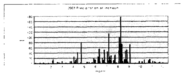
Fig. 1. Precipitation record of the year 2003 at Incheon.
