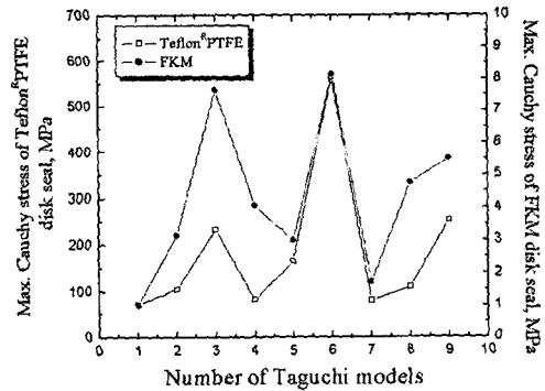
Fig. 6 Cauchy stress distributions of disk seal as a function of various Taguchi models.
