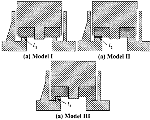
Fig. 1 Analysis models of SF 6 gas safety valve.
