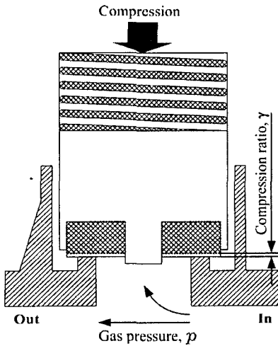
Fig. 2 Design parameters for optimization of disk-seal contact type cylinder using Taguchi method.
