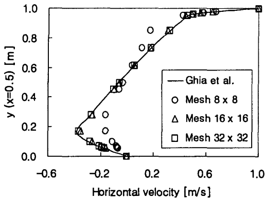
Fig. 8 A comparison of velocity solutions with Ghia, Ghia and Shin[8]
