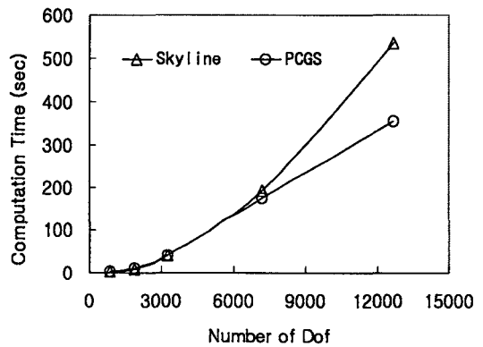
Fig. 6 Time comparison for lid-driven flow (quadratic elements, Re = 1000 )
