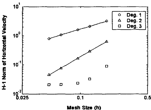
Fig. 2 Convergence trend for Kovaszny flow
