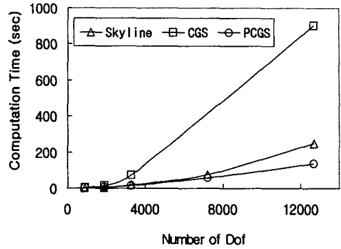
Fig. 3 Time comparison for Kovaszny flow (quadratic elements, Re = 40)
