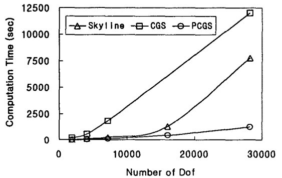
Fig. 4 Time comparison for Kovaszny flow (cubic elements, Re = 40)
