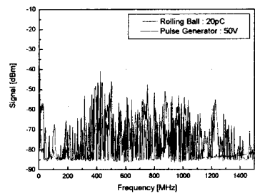
(a) 20pC-50V : D=19.9%
