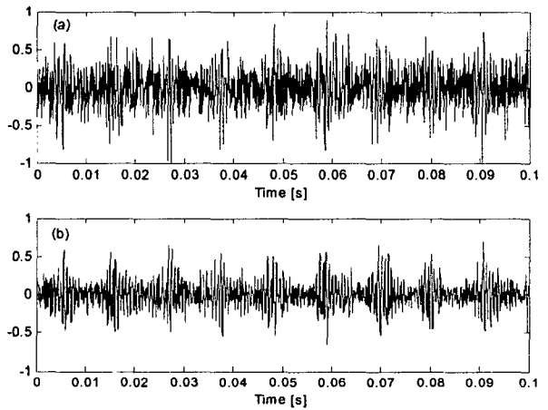
Fig. 6 Outer raceway defect
