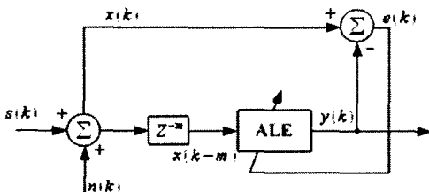
Fig. 2 Structure of ALE
