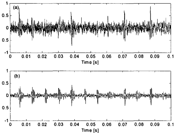
Fig. 8 Ball defect
