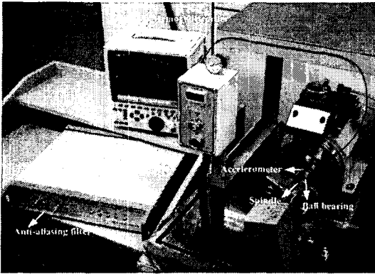
Fig. 5 Experimental set-up
