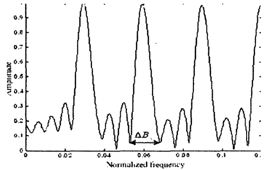
Fig. 4 Frequency response of ALE
