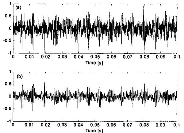
Fig. 7 Inner raceway defect
