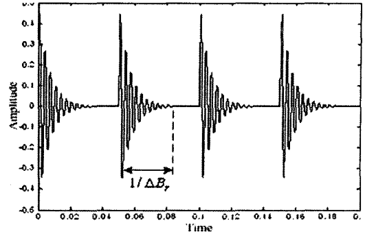
Fig. 3 Bearing defective signal in time domain
