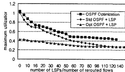
Figure 6. Comparison of route adaptation strategies
