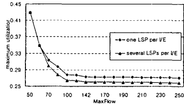
Figure 5. Maximum utilization over MaxFlow
