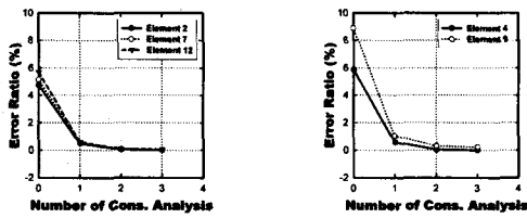
(a) Ridge cables (b) Upper ring cables
