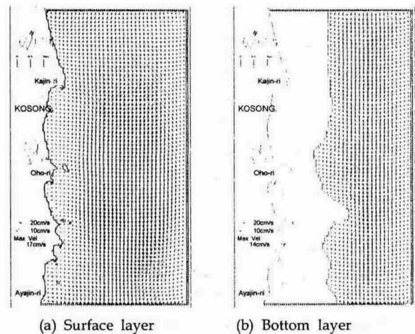
Fig. 9 Tidal current vector diagram on maximum flood flow in Neap tide.
