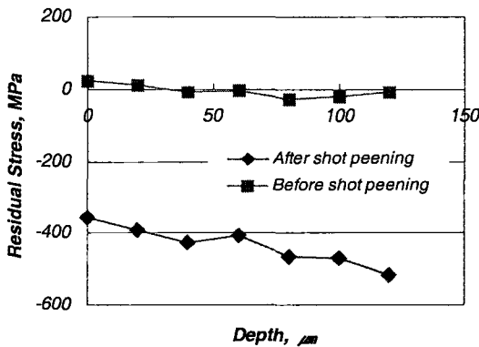
Fig. 8 Residual stress distribution
