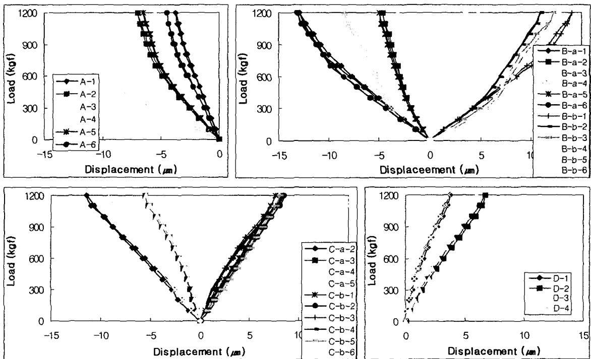
Fig. 10 Hysteresis curves for each positions of strain gauges in 1200kg test
