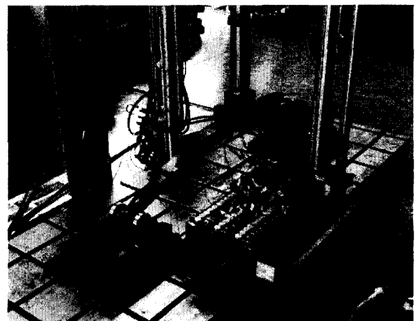
Fig. 5 Leaf spring assembly test
