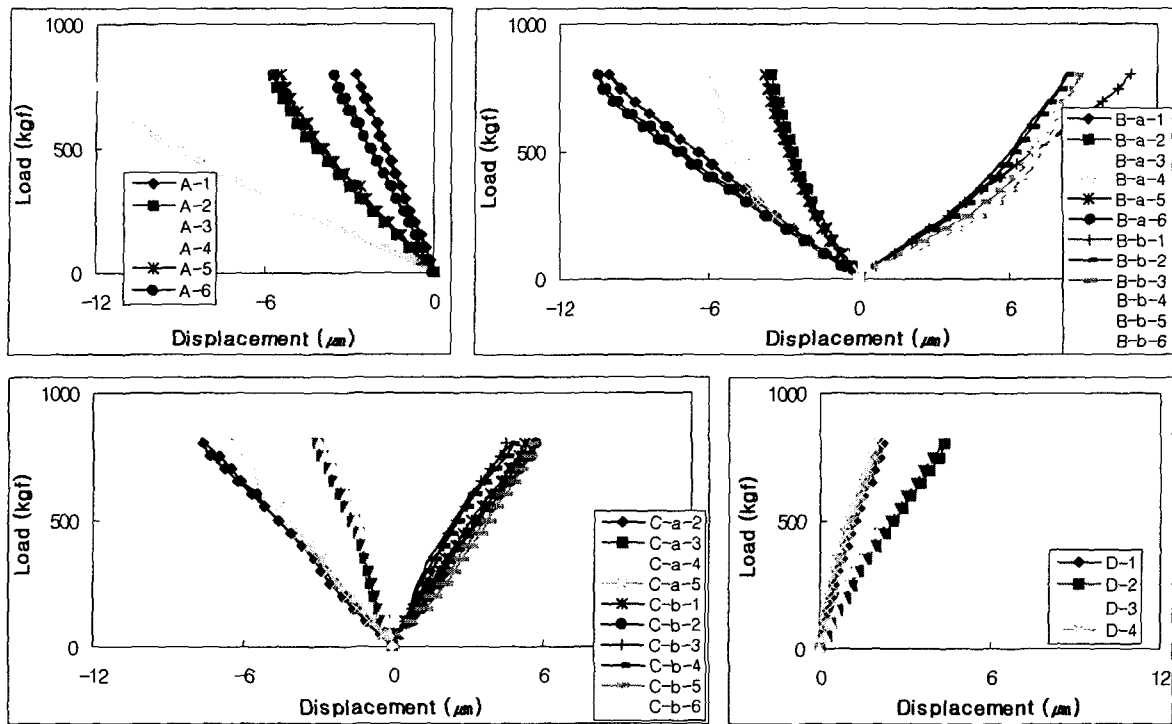
Fig. 9 Hysteresis curves for each positions of strain gauges in 800kg test
