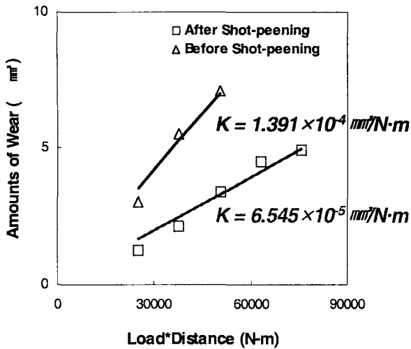
Fig. 7 Wear rate of specimens
