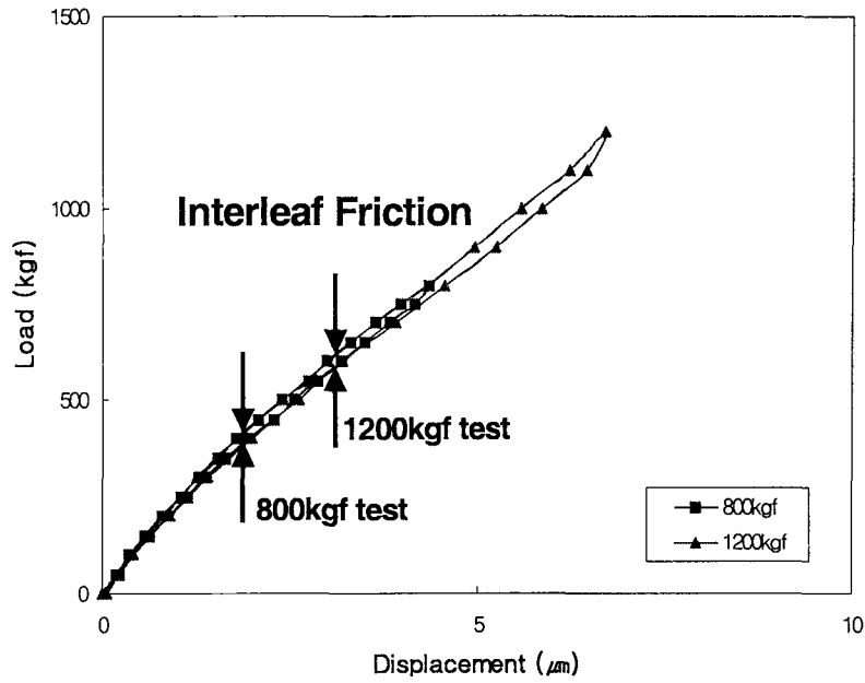
Fig. 11 Measurement of interleaf friction force
