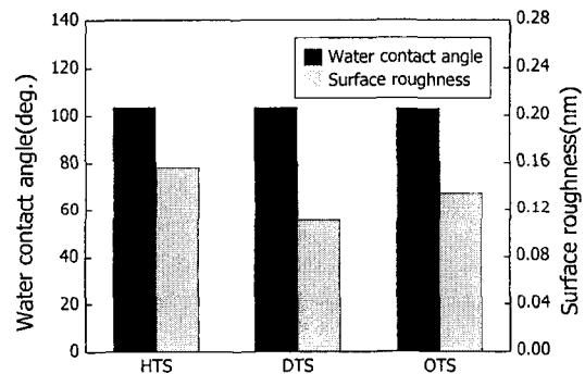
Fig. 5 Water contact angle and Surface roughness of SAM specimens with chain length.
