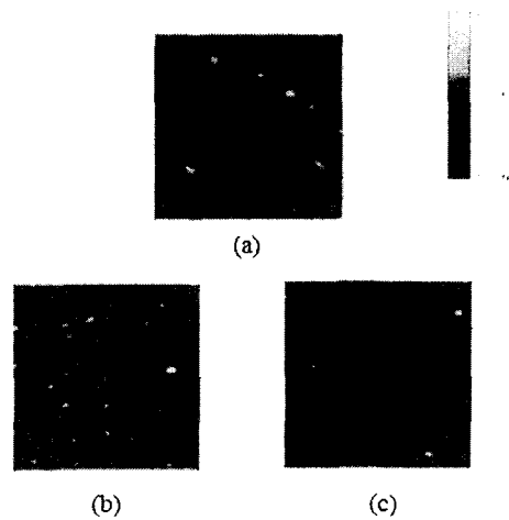
Fig. 4 2D topography of the SAM samples of (a) HTS SAM, (b) DTS SAM, and (c) OTS SAM.
