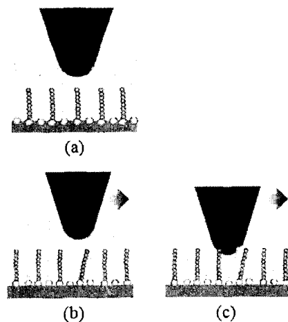
Fig. 11 Nano adhesion (a), nano friction (b) and micro friction (c) mechanism of mixed SAM.
