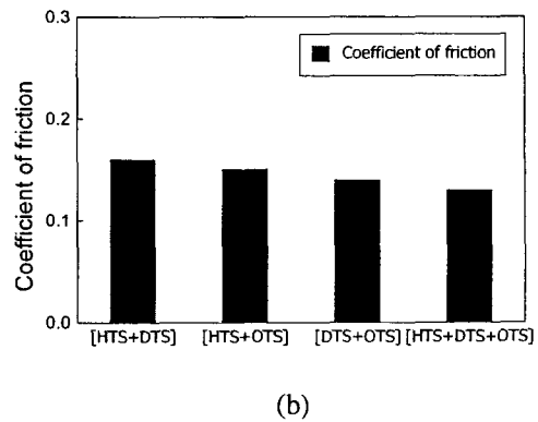
Fig. 9 (a) Nano adhesion forces and nano friction forces and (b) Micro friction coefficient of mixed SAM samples.
