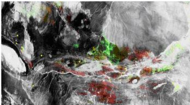
Fig.6. Alteration anomaly map of a copper deposit in Tuwu
