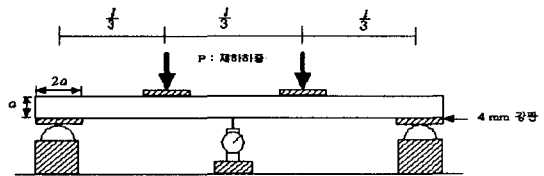
Fig. 1. Test Equipment 1)
