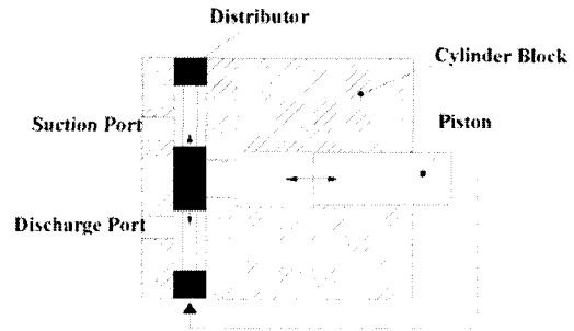
Fig. 3 Operating principle of a piston in an axial piston pump of bent axis.
