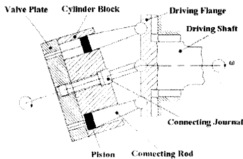
Fig. 1 Configuration of an axial piston pump of bent axis.
