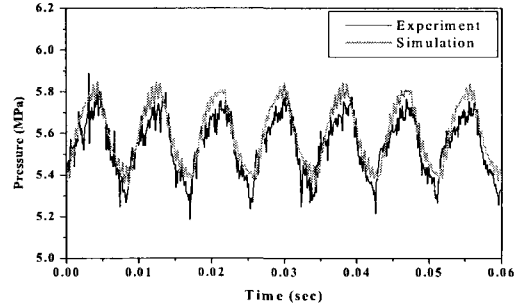
Fig. 6 Comparison of discharge pressure between simulation and experiment with rotational speed 1000rpm
