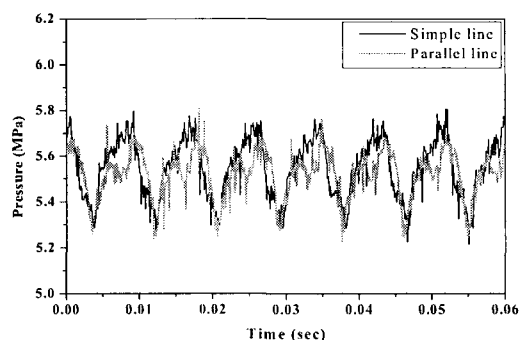
Fig. 7 Comparison of experimental results in inlet pressure between simple line and parallel line with rotational speed 1000rpm
