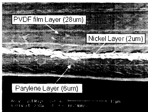
Fig. 2. Side view SEM image of the fabricated piezoelectric tactile sensor with parylene coating for showing the details of the piezo, nickel, and coated parylene.
