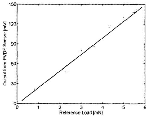
Fig. 5. Calibration result of the miniaturized PVDF sensor (2*6 mm) for load input.
