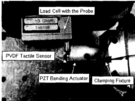
Fig. 4. Experimental setup for analyzing the performance of the PVDF sensor with parylene coating
