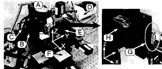
A : Optical Stereo Microscope (Top View) E : Fine Motion Stage B : Optical Microscope (Global View) F : Coarse Motion Stage C : Optical Microscope (Lateral View) G : Micro Gripper D : Illuminator Source H : Opto-electrical Component
