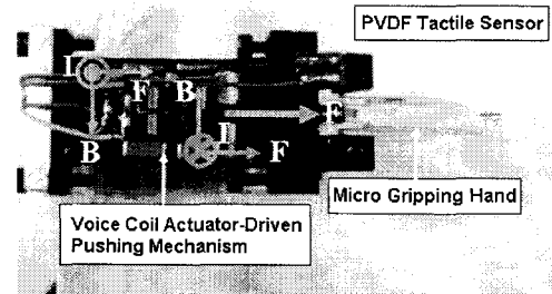
Fig. 1. A tactile sensor integrated microgripper and its operational principle actuated by voice coil motors.
