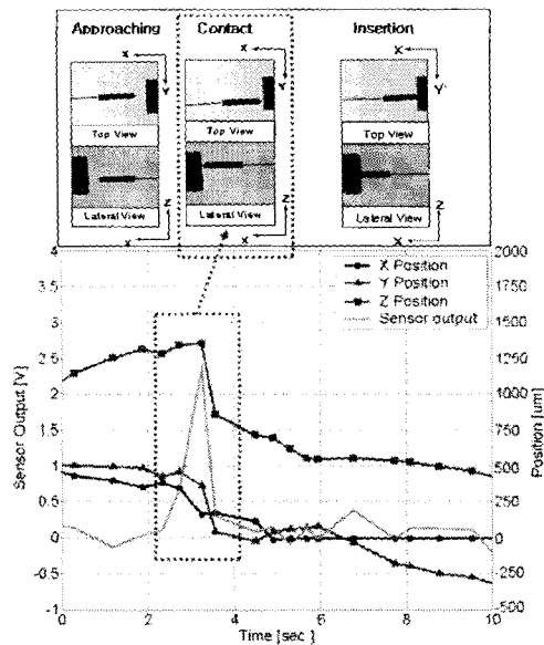
Fig. 7. Experimental result of the force feedback-based microassembly.
