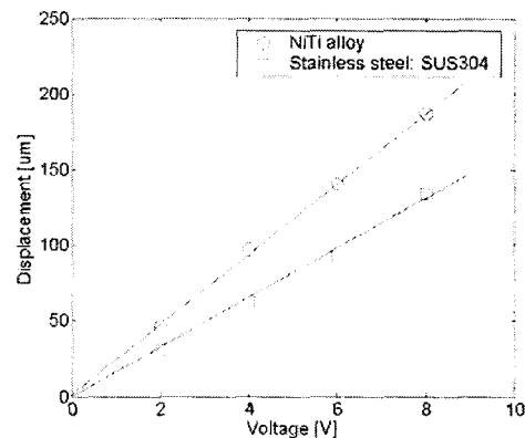
Fig. 3. Experimental result of gripping stroke for a 1 Hz square wave.
