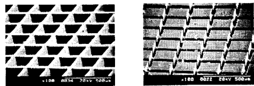
(a) Silicone rubber (b) Polyethylen glycol pad Fig. 7 SEM image of silicone rubber and polishing pad
