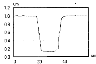
Fig. 4 Shape of 20 \mu\text{m} pattern on silicone rubber
