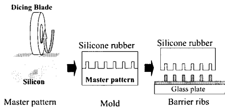
Fig. 8 Manufacturing process of PDP barrier ribs
