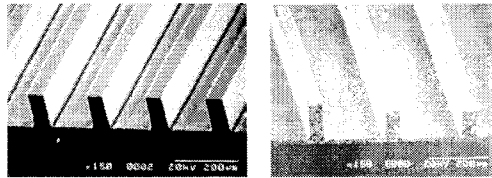
(a) Master (b) PDP barrier ribs Fig. 9 Master and PDP barrier ribs
