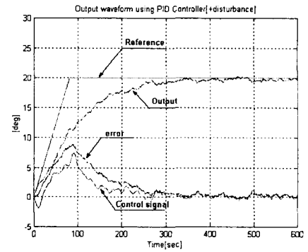
(b) (+) disturbance
