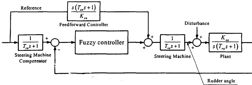
Fig. 2 . System of Ship using Fuzzy Controller
