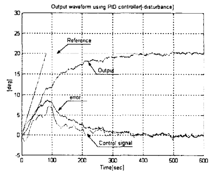
(c) (-) disturbance
