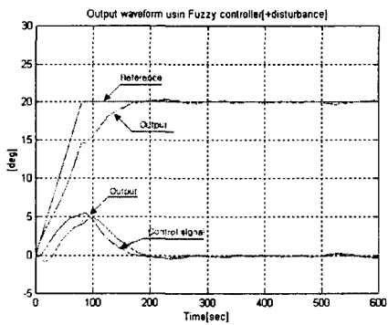
(c) (-) disturbance
