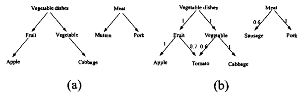
Figure 1. Exact Taxonomies and Fuzzy Taxonomies.
