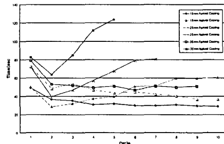
Fig. 9 Response time of SMA actuator displacement
