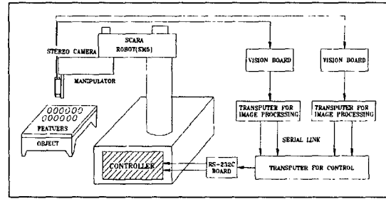
Fig. 9. Schematic diagram of visual feedback system
