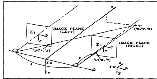
Fig. 10. The coordinates system of stereo vision model
