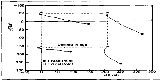
Fig. 11. Trajectories of the Feature Point on the image (Monocular)
