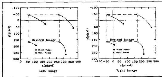
Fig. 12. Trajectories of the Feature Point on the image (Stereo)
