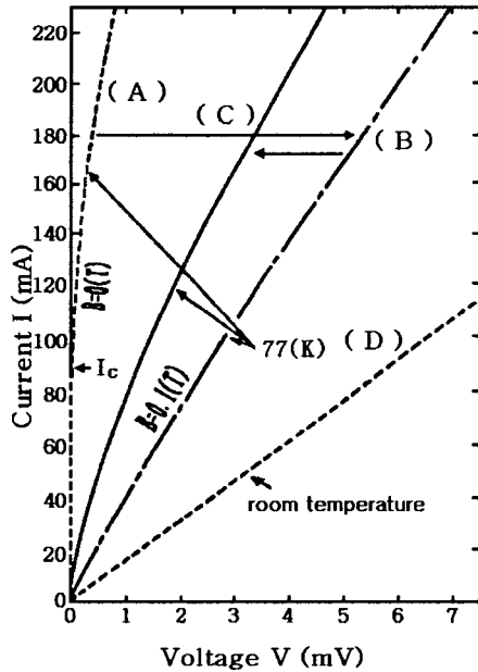
Fig. 1. Current-voltage characteristics of the BPSCCO ceramics.
