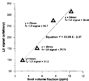
Fig. 11 LII signal vs soot volume fraction obtained from extinction experiments.
