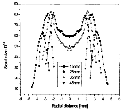
Fig. 12 Mean diameters of soot particles (D 30 ) measured using a light extinction/scattering method.
