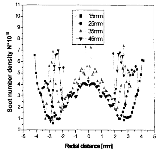
Fig. 13 Number density of soot particles measured using a light extinction/scattering method.
