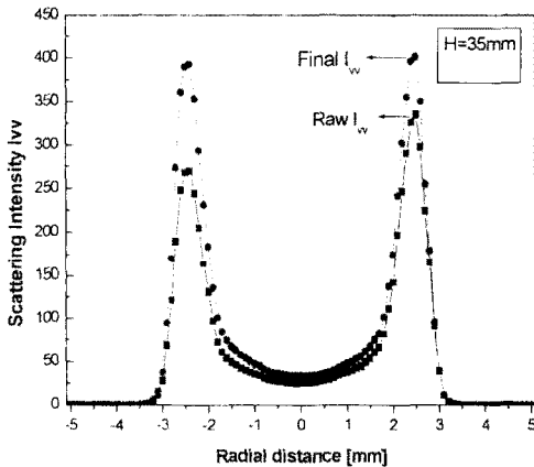
Fig. 5 Light scattering data before and after correction for laser beam attenuation and signal trapping.
