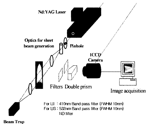
Fig. 2 LII measurement set-up.
