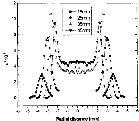
Fig. 9 Soot volume fractions measured by laser extinction method.
