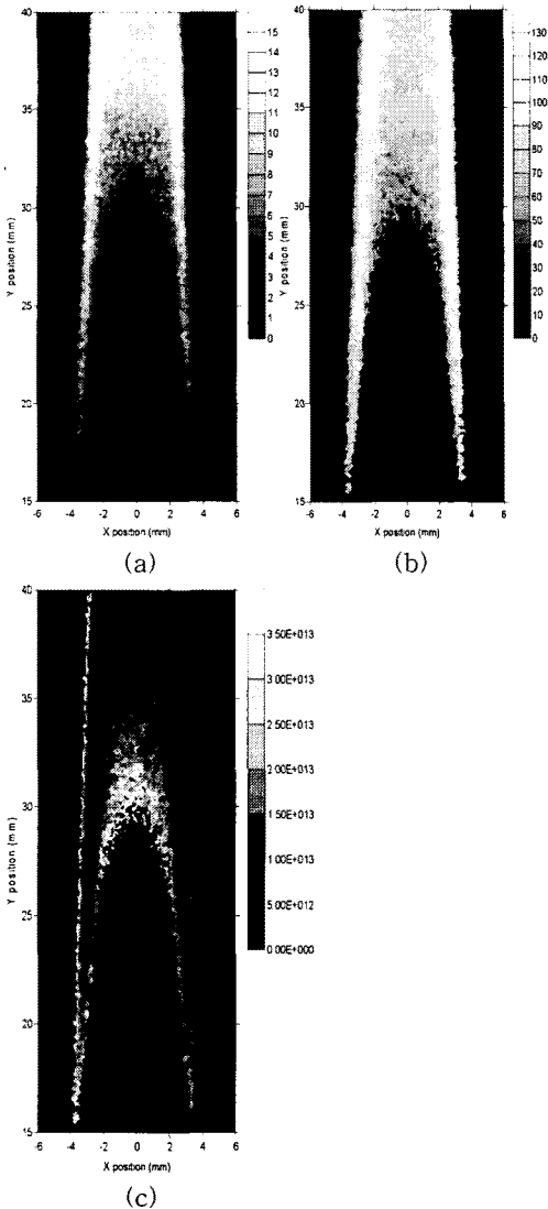
Fig. 14 Simultaneous 2-D LII/LIS measurements (a) soot volume fraction (ppm), (b) mean diameter( D_{63} ) and (c) number density.
