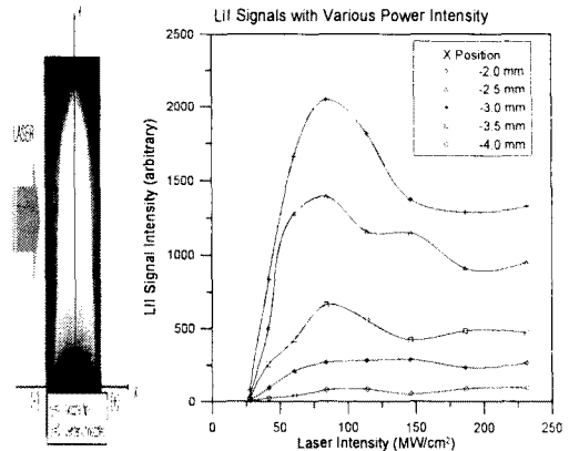
Fig. 6 Characteristics of LII signal with various laser power conditions.
